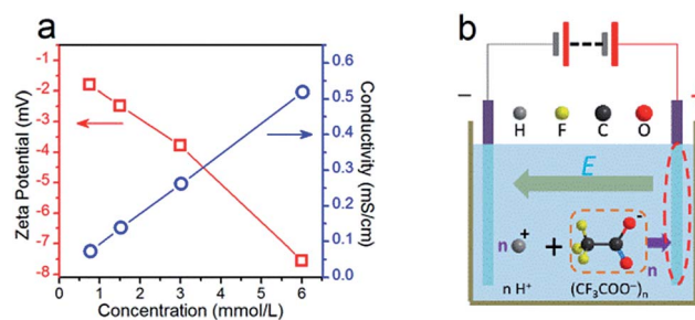
Fig. 1 (a) Zeta potential and conductivity of TFA solutions at various concentrations. (b) Schematic of electrophoretic deposition system for TFA films.
