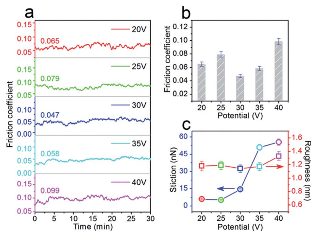
Fig. 3 (a) Friction coefficient vs. time curves of the films deposited at different voltages (20–40 V). Conditions for friction experiments: load = 20 mN, sliding velocity = 0.01 \text{ m s}^{-1} . (b) Friction coefficient of the films as a function of voltage. (c) Stiction and roughness of the films as a function of voltage.
