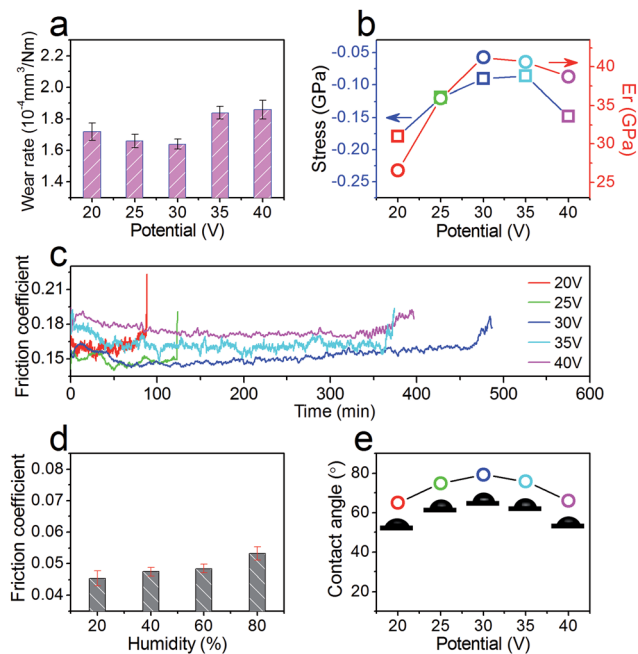
Fig. 4 (a) Wear rate, (b) internal stress and elastic modulus, and (c) wear life of the films deposited at different voltages (20–40 V). (d) Friction coefficient of the film deposited at 30 V as a function of humidity. (e) Contact angle of the films deposited at different voltages (20–40 V).
