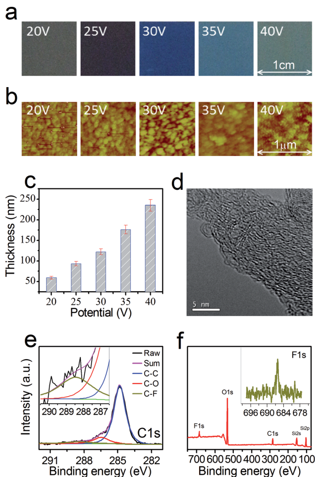
Fig. 2 (a) Optical and (b) AFM images of the films deposited at different voltages (20–40 V). (c) Thicknesses of the films as a function of voltage. (d) TEM image of the film deposited at 30 V. (e) C 1s (inset is an enlarged image of the C–F bond) and (f) XPS full spectrum of the film deposited at 30 V (inset is the corresponding F 1s spectrum).
